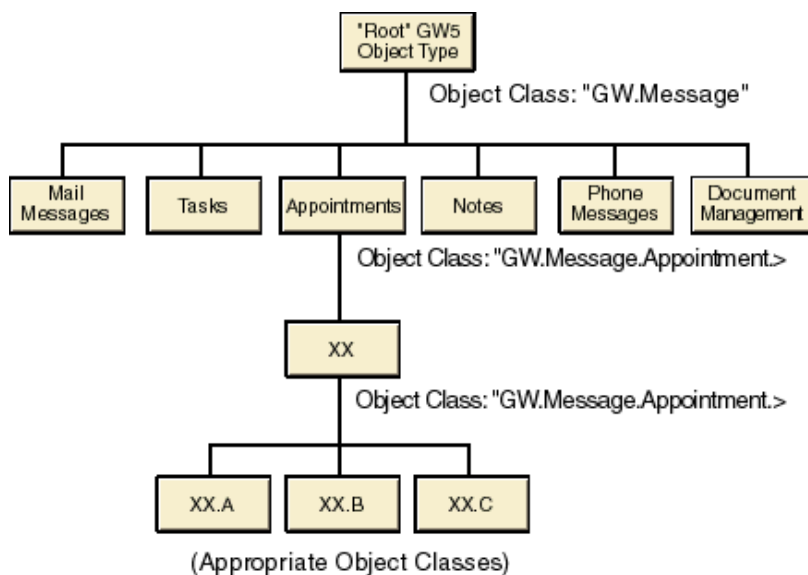
Figure 1-1 C3PO Object Class Hierarchy
