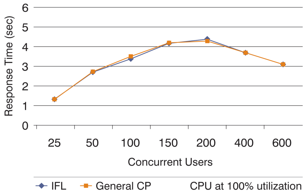
Figure 1. IFL vs. General CP
