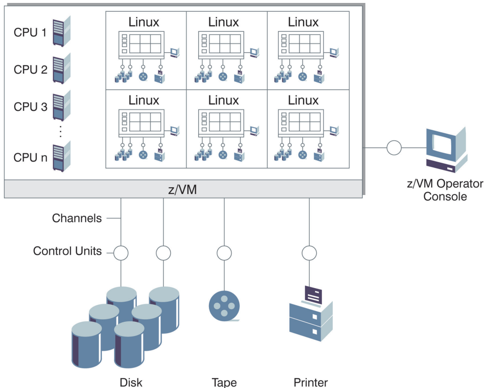
Figure 2. z-VM OperatorConsole
