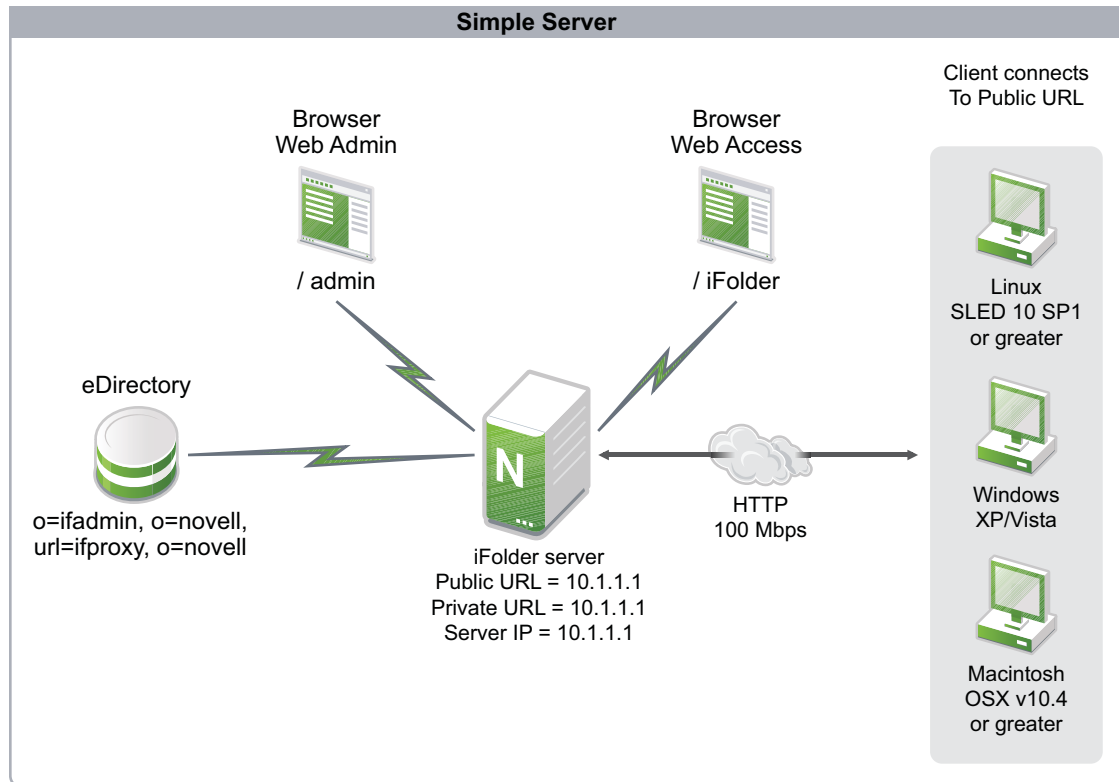
Figure 2-1 Single Server
