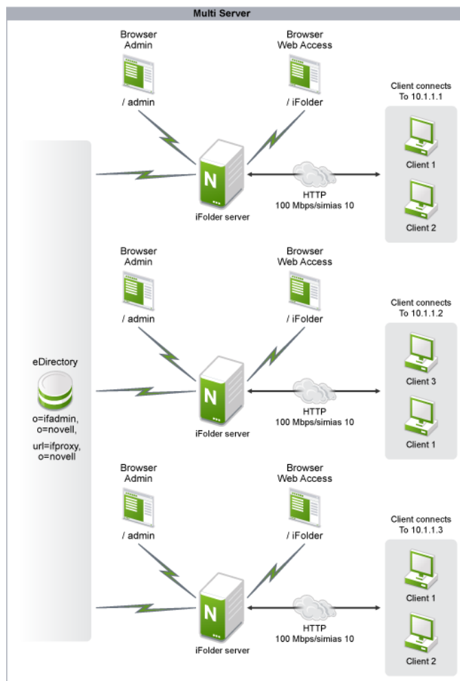
Figure 4-1 Multi Server
