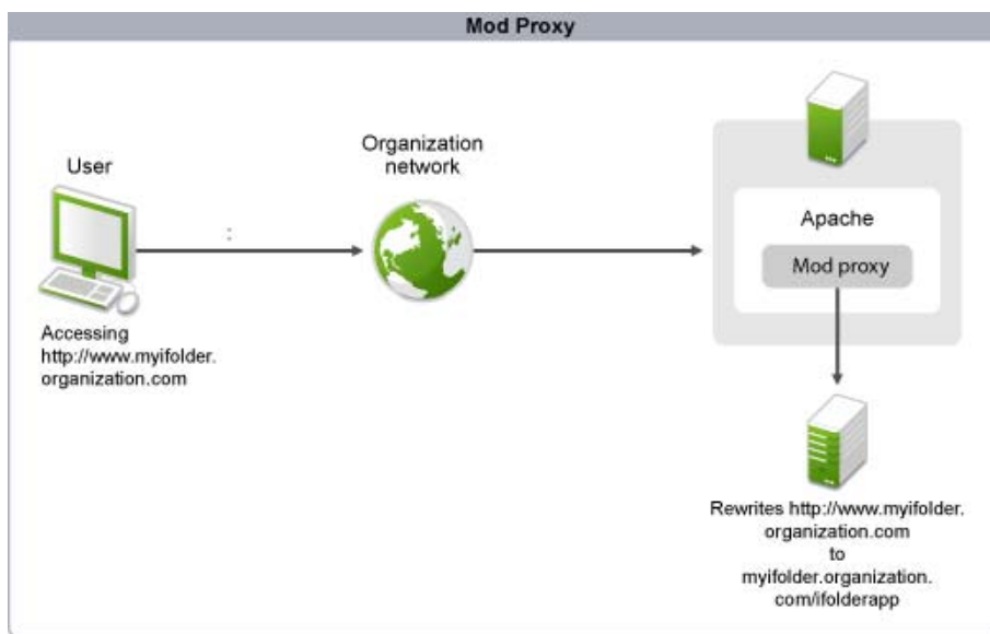
Figure 12-2 Mod Proxy
