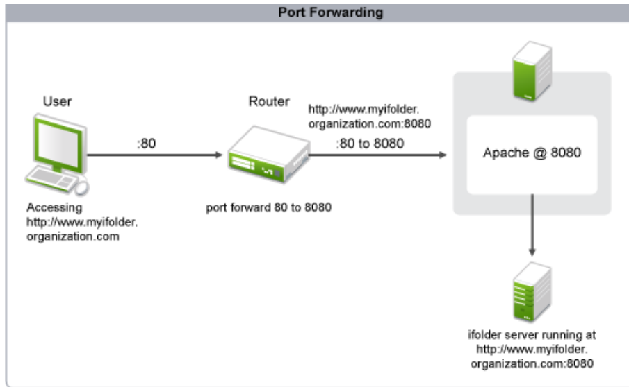
Figure 12-1 Port Forwarding
