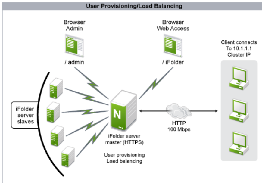
Figure 8-1 Load Balancer
