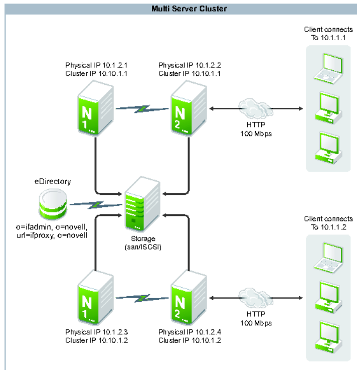
Figure 7-1 Multi-Server Cluster
