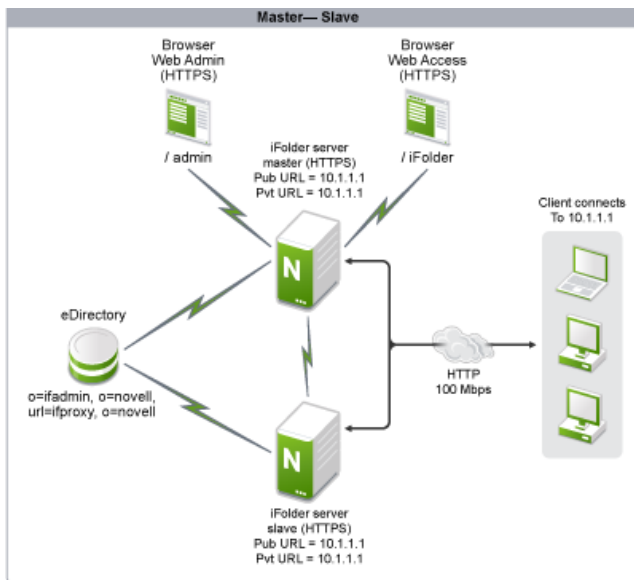
Figure 3-1 Master-Slave
