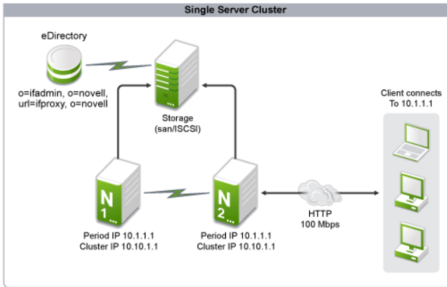
Figure 6-1 Single-Server Cluster
