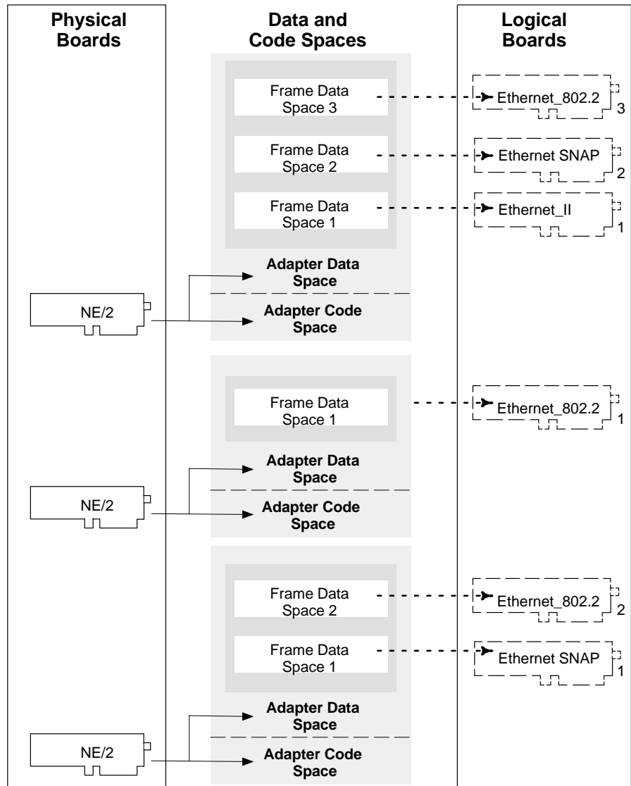
Figure 3.1 Implementation of Multiple Frame Support in Ethernet Topology
