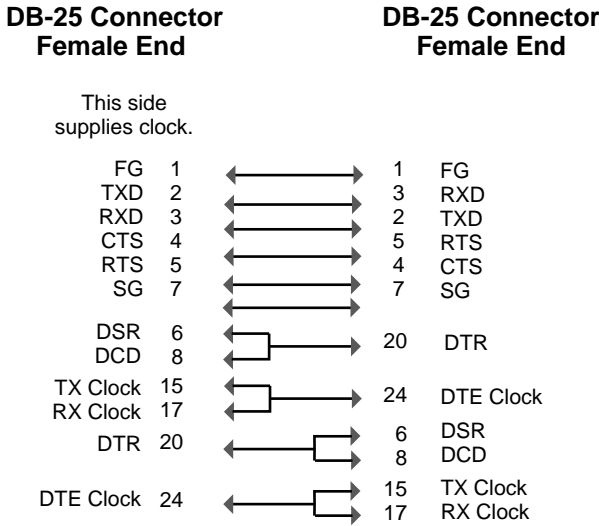
Figure 3 RS-232 Crossover Cable
