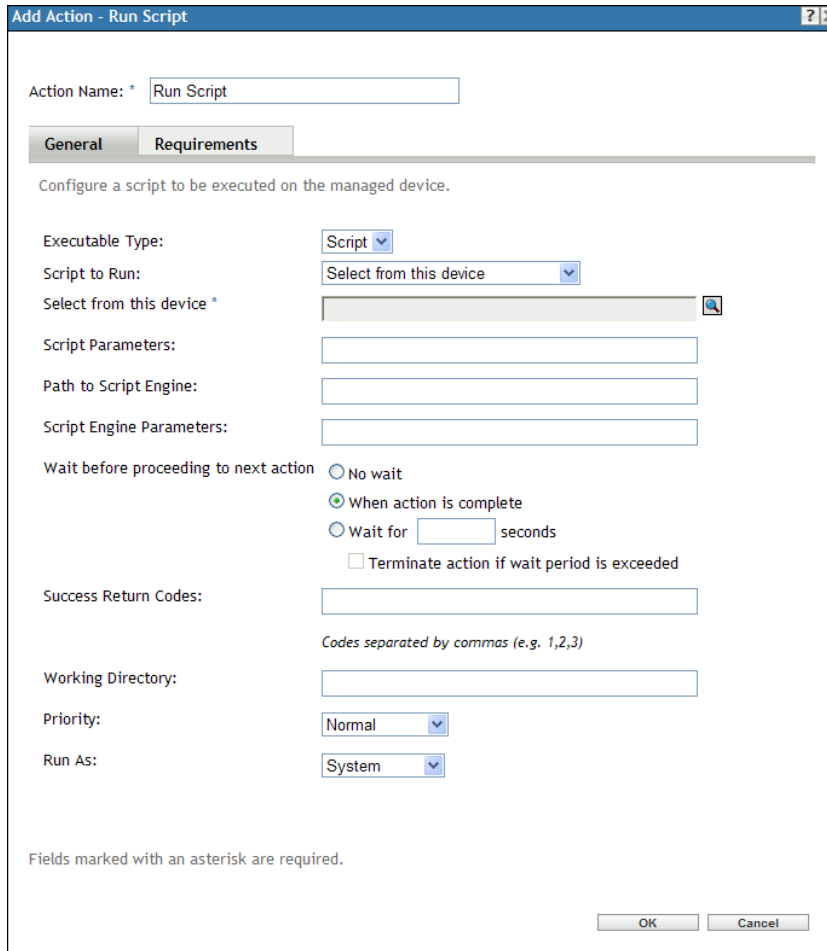
Figure 6-33 Action - Run Script Dialog Box with the Select From This Device option selected
