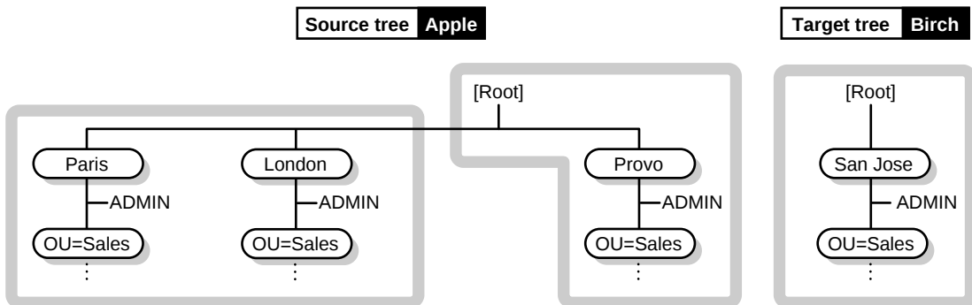
Figure 2 Directory Trees before a Merge
