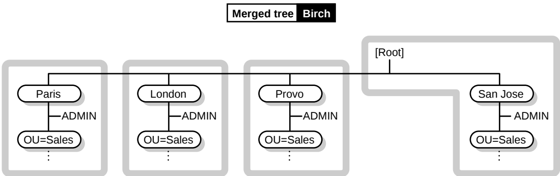
Figure 3 Directory Tree after a Merge
