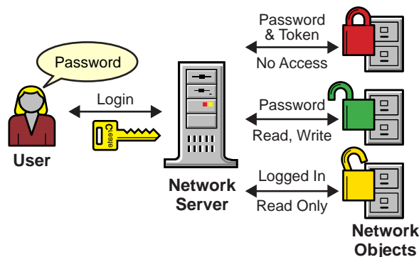
Figure 1 Single-Factor Authentication
