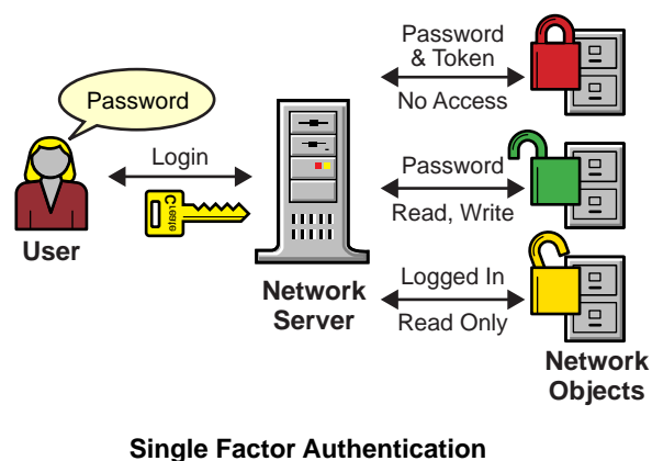
Figure 1 Single-Factor Authentication
