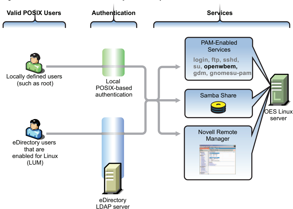
Figure 15-1 LUM Provides POSIX Access for eDirectory Users
