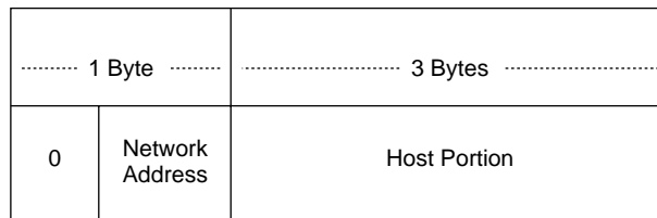
Figure 6 Class A IP Address
