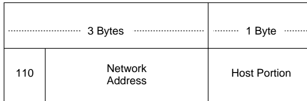
Figure 8 Class C IP Address
