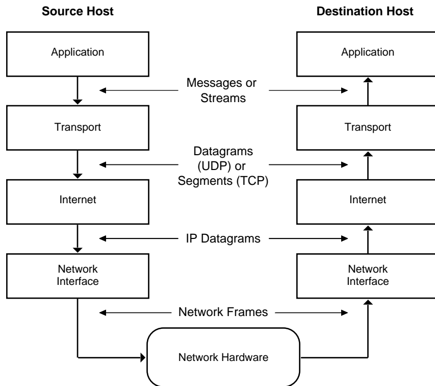
Figure 2 TCP/IP Model
