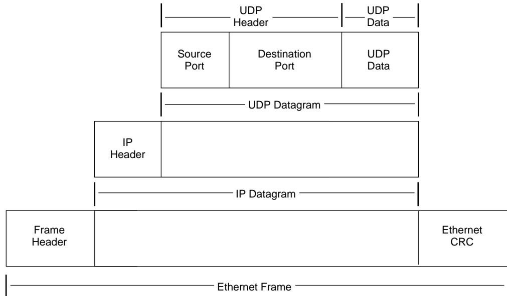
Figure 3 UDP Datagram Encapsulation
