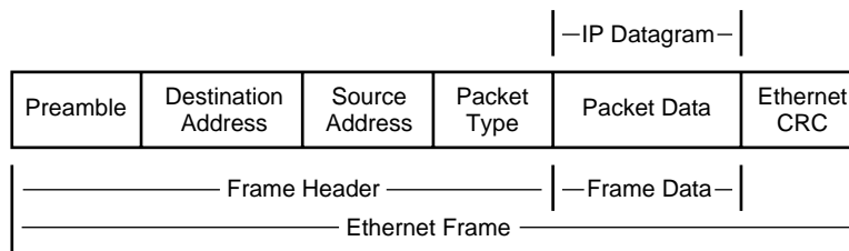
Figure 9 Packet Encapsulated in an Ethernet Frame
