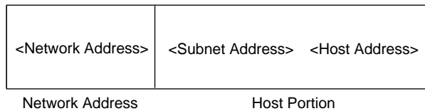
Figure 10 4-byte IP Address
