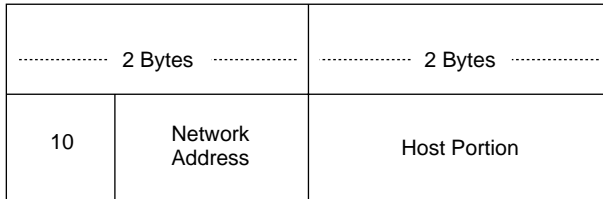
Figure 7 Class B IP Address
