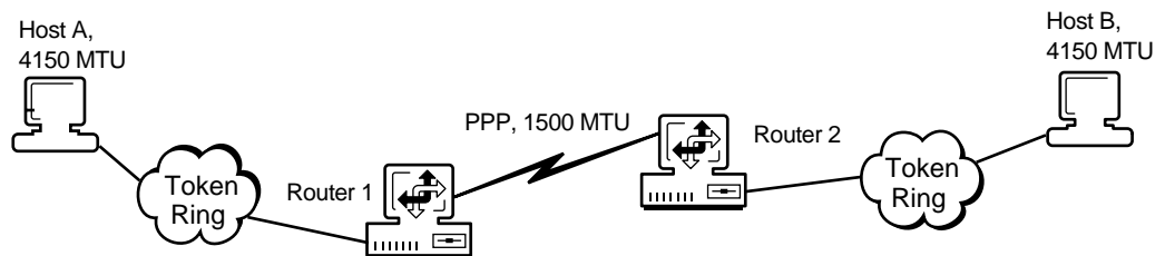
Figure 5 Sample Path MTU Discovery Process
