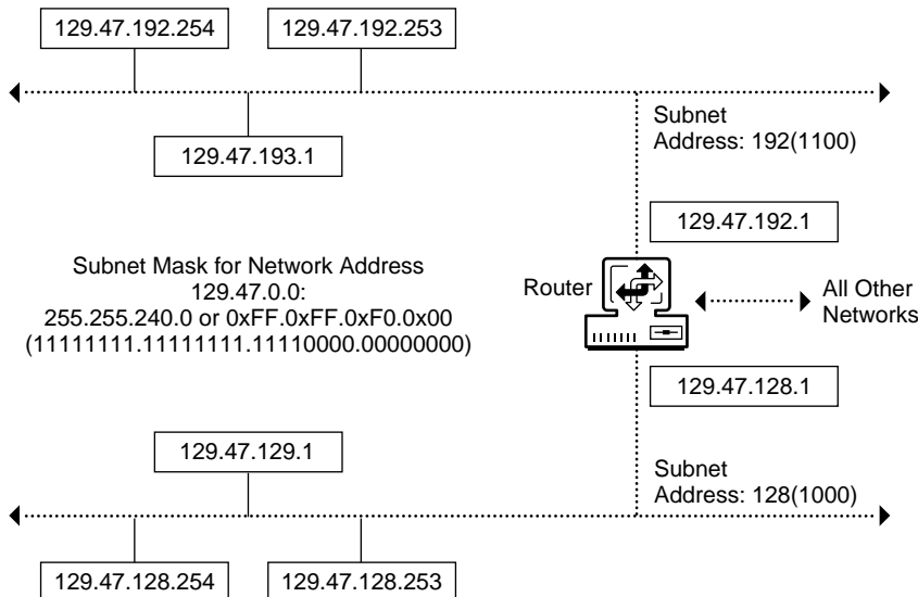
Figure 11 Single IP Network Divided into Two Subnets
