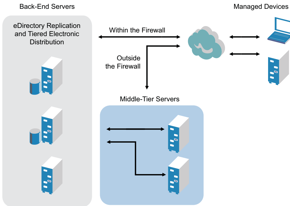
Figure 2-1 ZENworks Desktop Management Architecture
