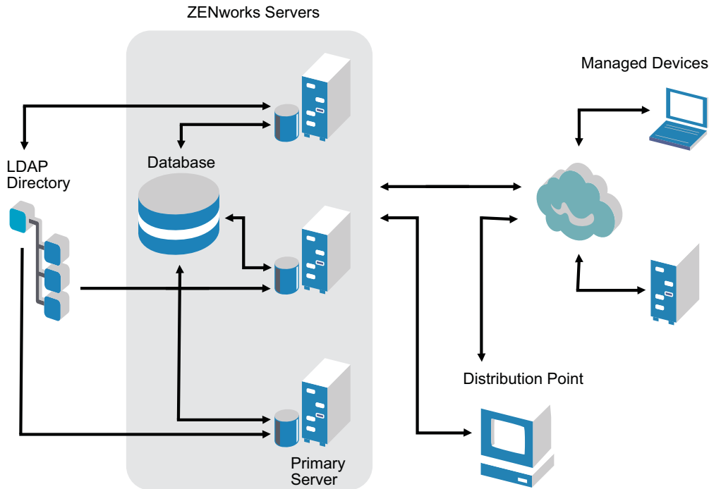
Figure 2-4 ZENworks 11 SP3 Architecture
