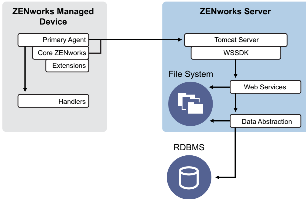
Figure 2-3 ZENworks 11 SP3 Client-Server Architecture
