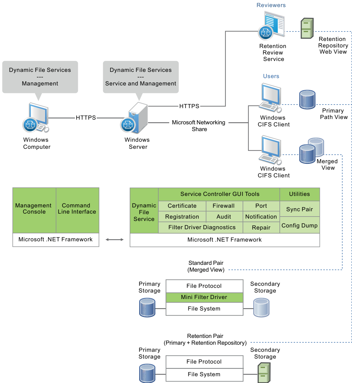
Figure 1-1 Dynamic File Services Software Components
