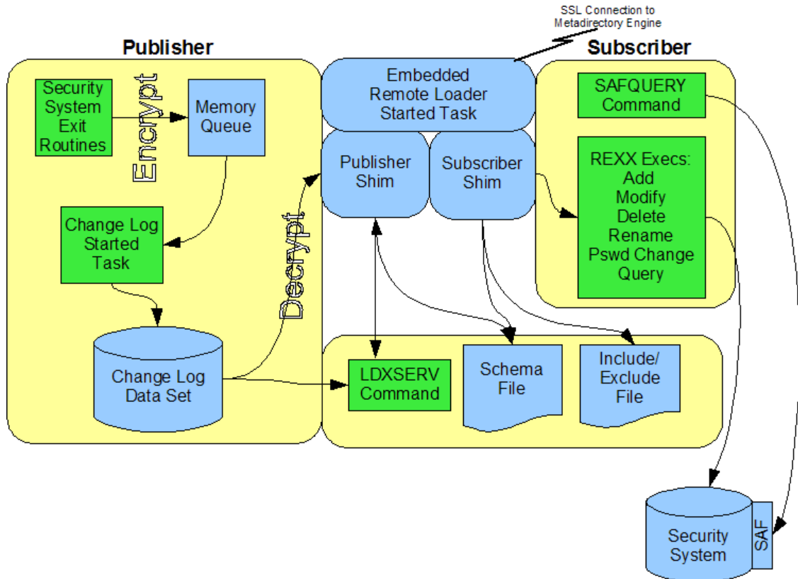
Figure 1-1 CA-Top Secret Driver Architecture
