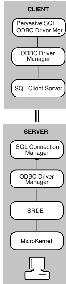
Figure 5-8 Pervasive.SQL 2000i Relational Architecture: Client
