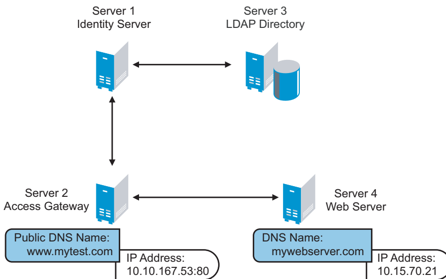
Figure 1-2 Basic Configuration
