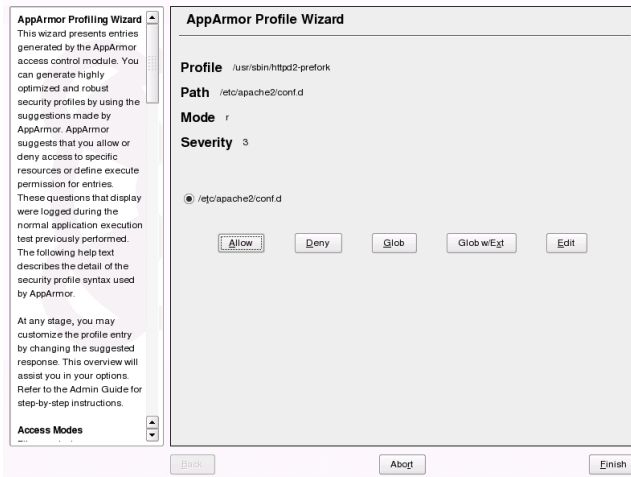
Figure 3.2 Learning Mode Exception: Controlling Access to Specific Resources
