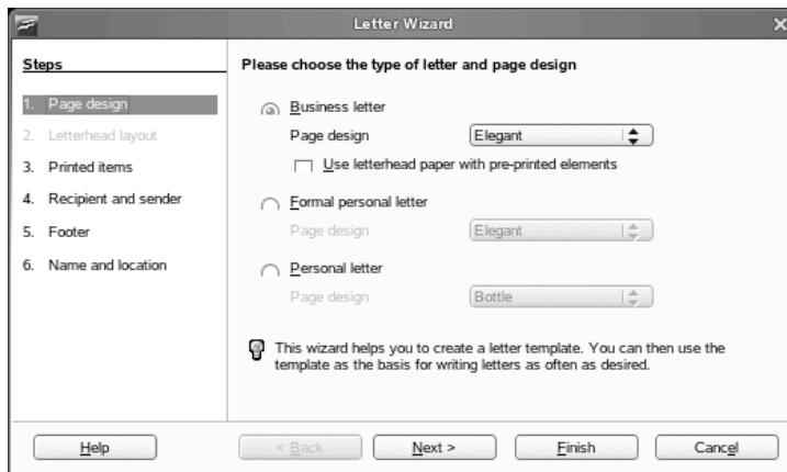
Figur 3.2 En OpenOffice.org-veiviser
