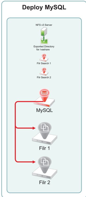
Figure 4-6 Deploying MySQL
