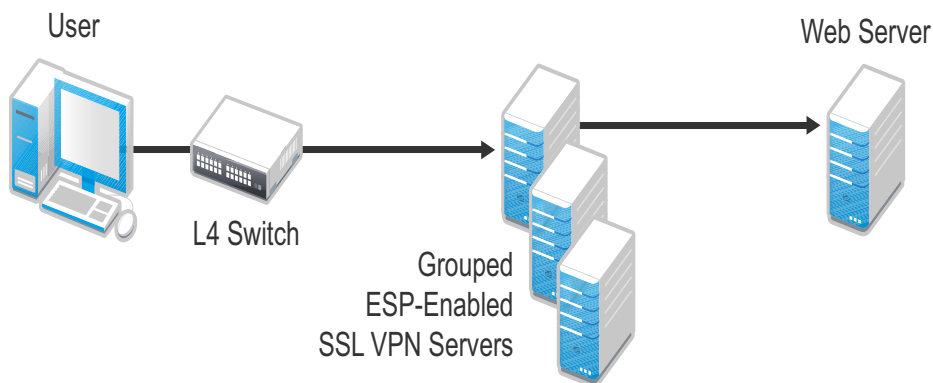
Figure 5-1 Cluster of SSL VPNs behind an L4 switch,
