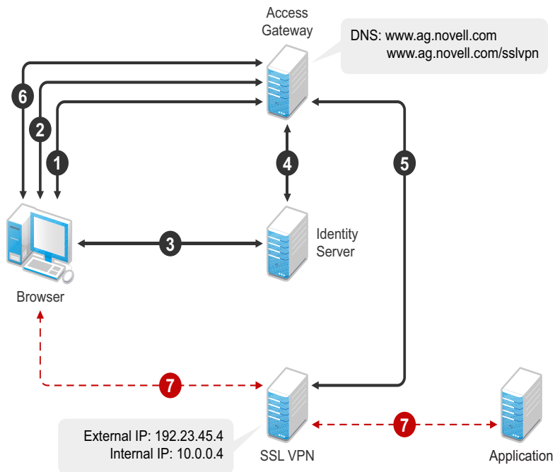
Figure 1-1 Traditional Novell SSL VPN
