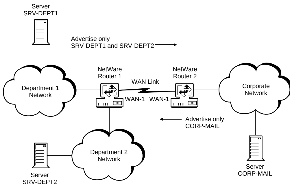
Figure 2 IPX SAP Filter Example
