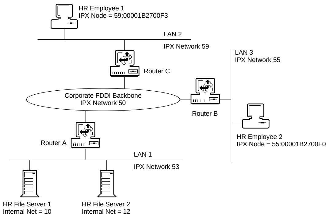
Figure 4 IPX Packet Forwarding Filter Example
