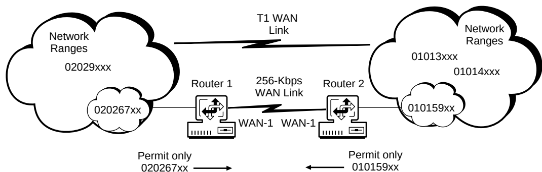
Figure 3 IPX Routing Information Filter Example
