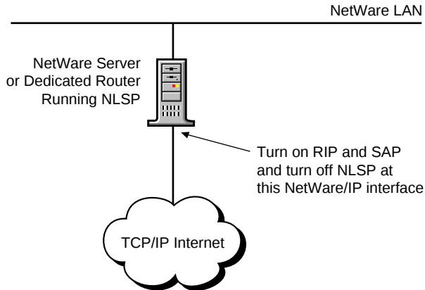
Figure 9 Configuring an Interface for NetWare/IP
