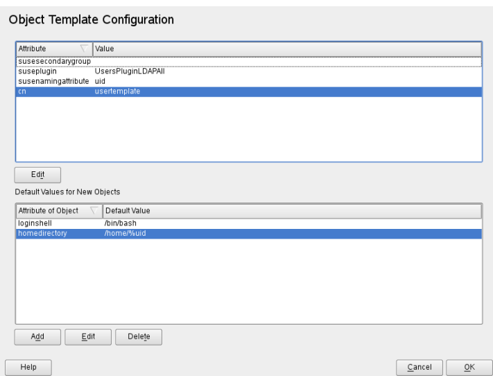
Figure 20.6 YaST: Configuration of an Object Template
