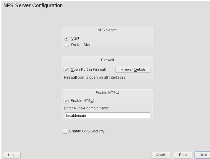
Figure 21.2 NFS Server Configuration Tool
