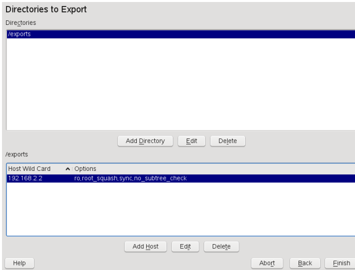
Figure 21.5 Exporting Directories with NFSv2 and v3
