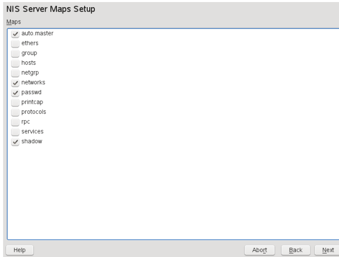
Figure 19.4 NIS Server Maps Setup
