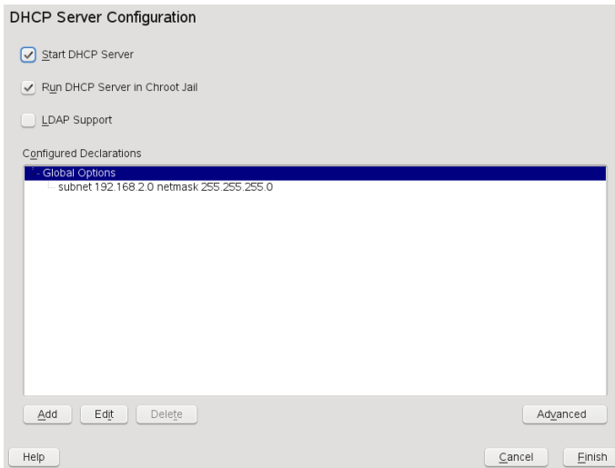
Figure 17.6 DHCP Server: Chroot Jail and Declarations
