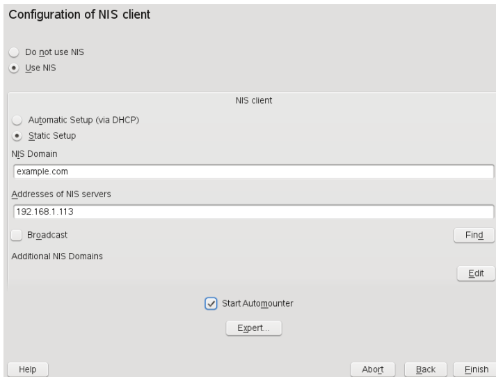
Figure 19.6 Setting Domain and Address of a NIS Server
