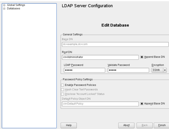
Figure 20.2 YaST LDAP Server Configuration
