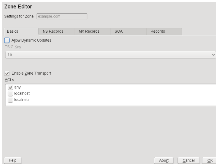
Figure 16.5 DNS Server: Slave Zone Editor
