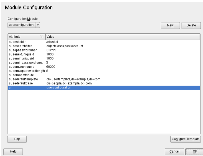
Figure 20.5 YaST: Module Configuration
