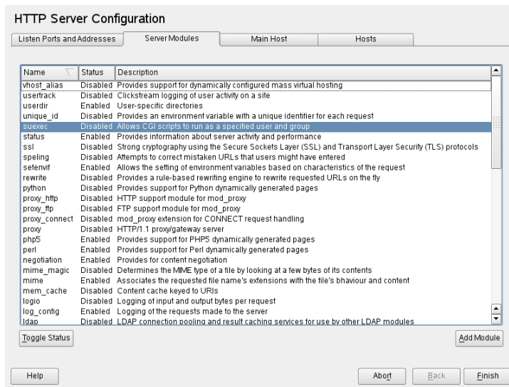
Figure 22.4 HTTP Server Configuration: Server Modules
