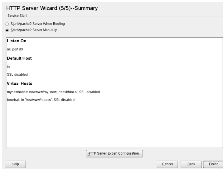
Figure 22.2 HTTP Server Wizard: Summary
