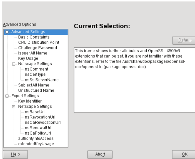
Figure 30.4 YaST CA Module—Extended Settings
