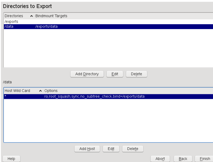
Figure 21.4 Exporting Directories with NFSv4
