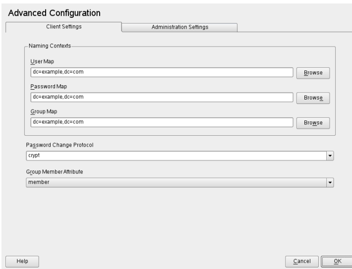
Figure 20.4 YaST: Advanced Configuration
