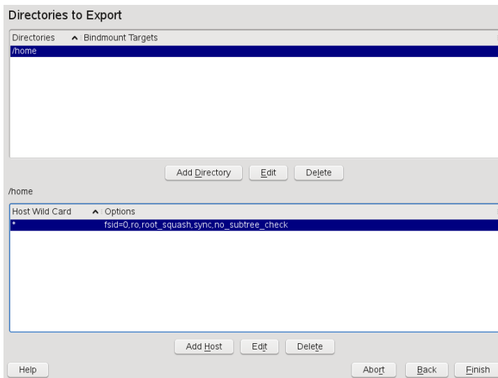
Figure 21.3 Configuring an NFS Server with YaST
