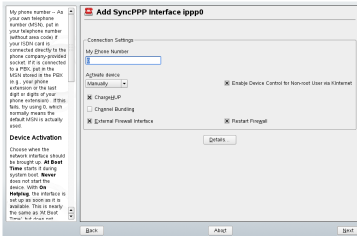
Figure 14.6 ISDN Interface Configuration
