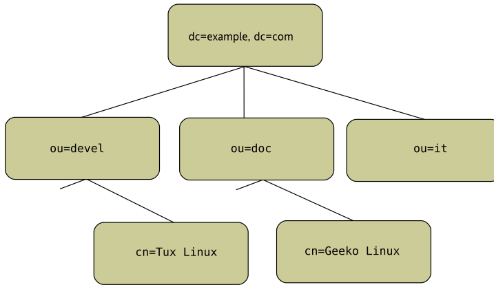
Figure 20.1 Structure of an LDAP Directory
