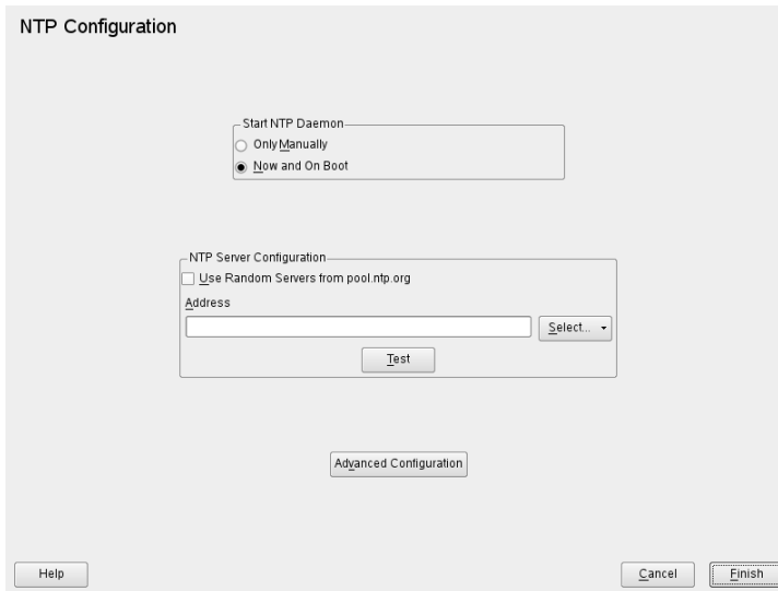
Figure 18.1 YaST: NTP Configuration
