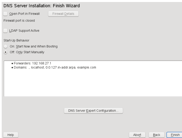
Figure 16.3 DNS Server Installation: Finish Wizard
