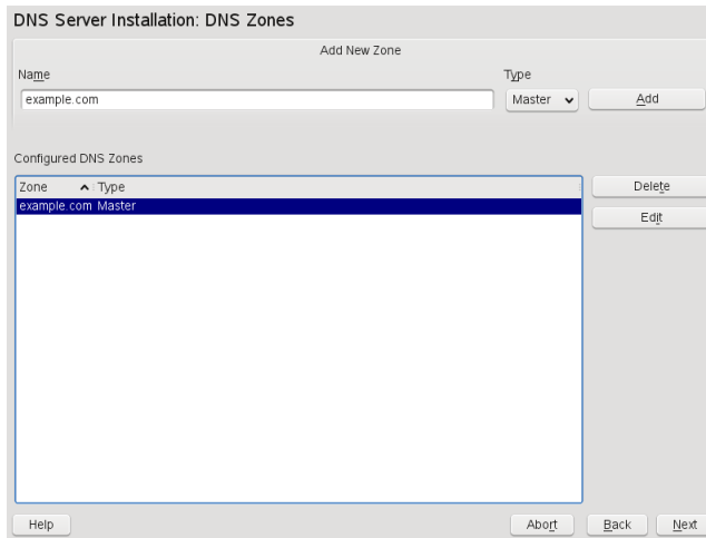
Figure 16.2 DNS Server Installation: DNS Zones
