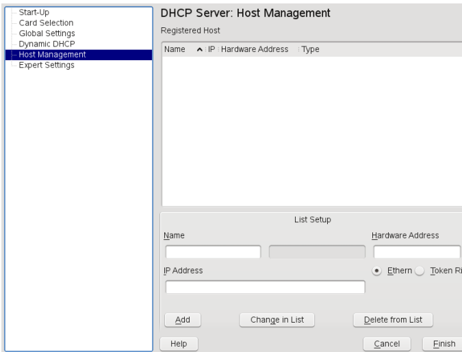
Figure 17.5 DHCP Server: Host Management
