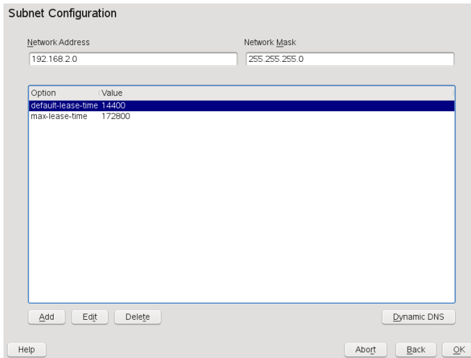
Figure 17.8 DHCP Server: Configuring Subnets
