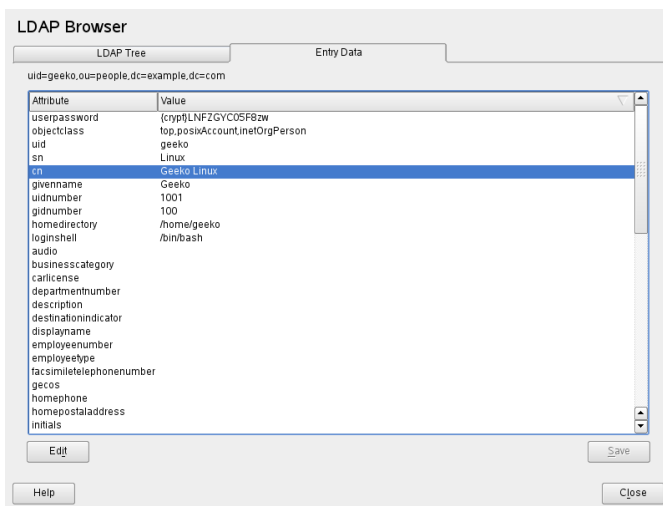
Figure 20.9 Browsing the Entry Data
