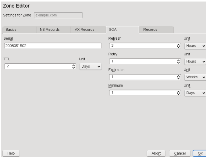
Figure 16.8 DNS Server: Zone Editor (SOA)
