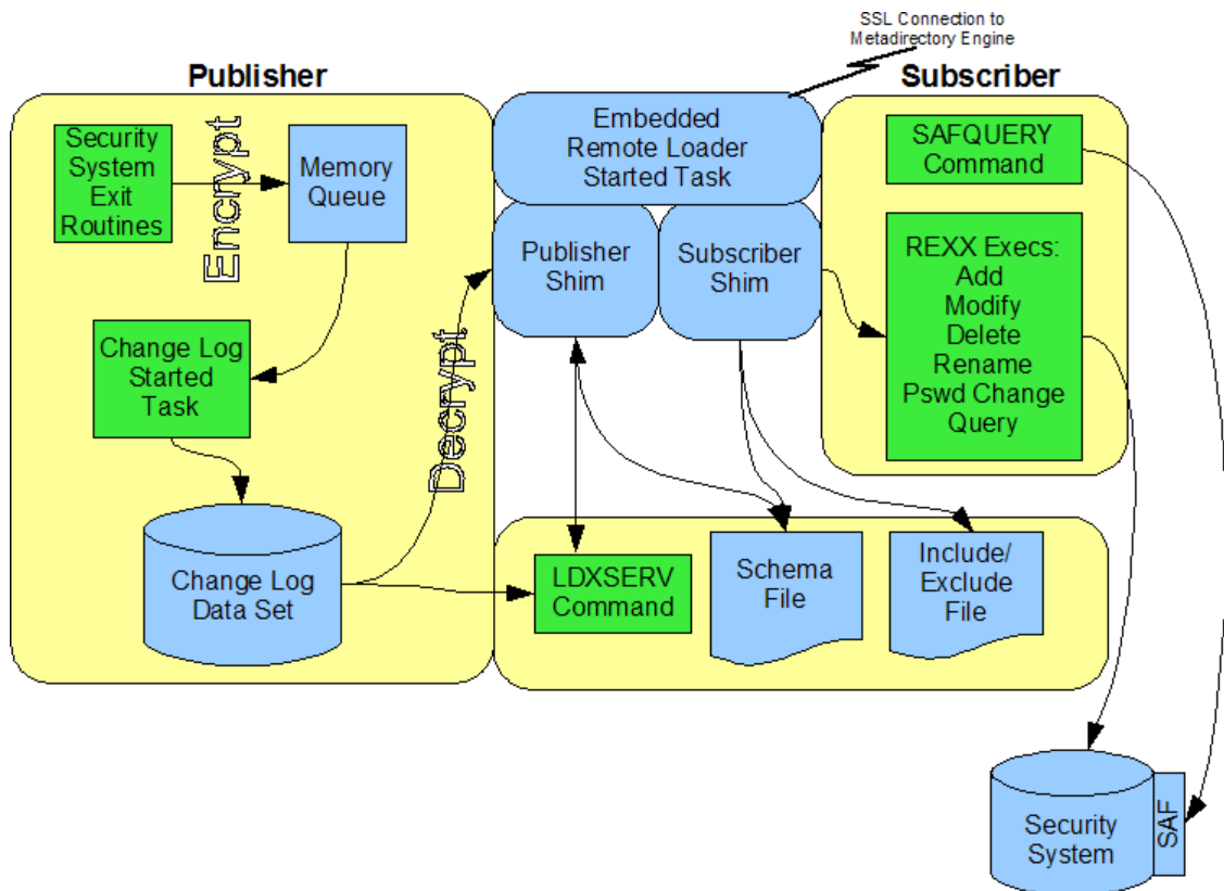
Figure 2-1 CA-Top Secret Driver Architecture
