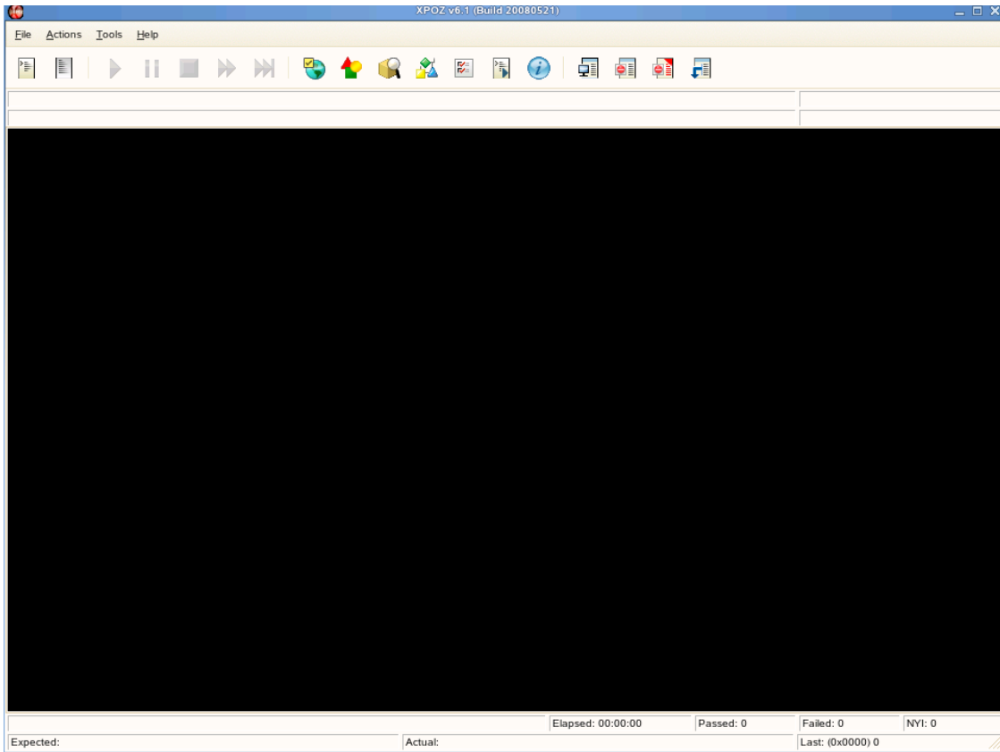
Figure 5-1 XPOZ GUI
