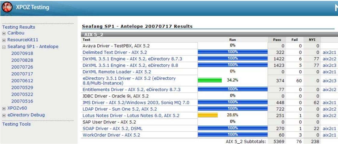
Figure 6-1 XPOZ Results Web Page Layout
