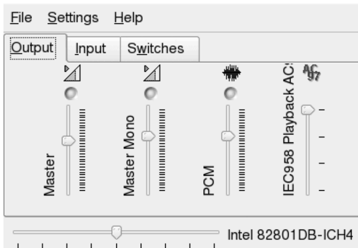
Figur 1.19 KMix-mixern
