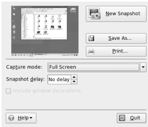
Figur 1.18 KSnapshot
