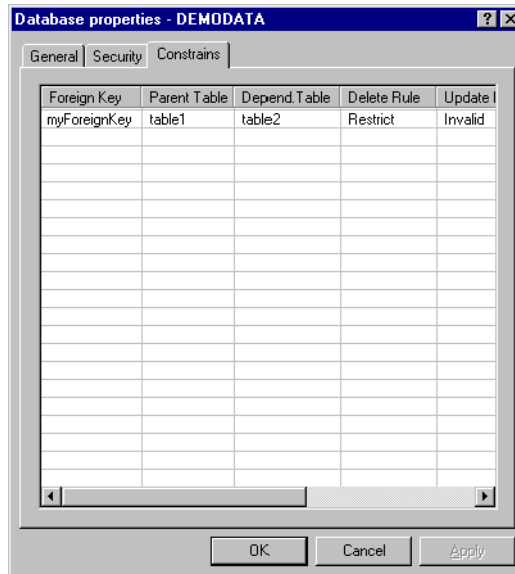
Figure 3-34 Database Properties
