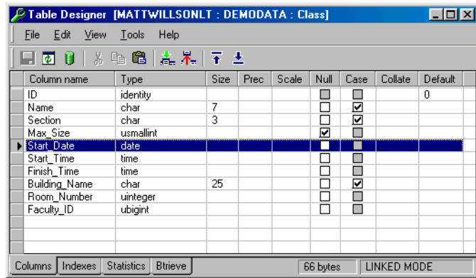
Figure 3-14 Table Designer
