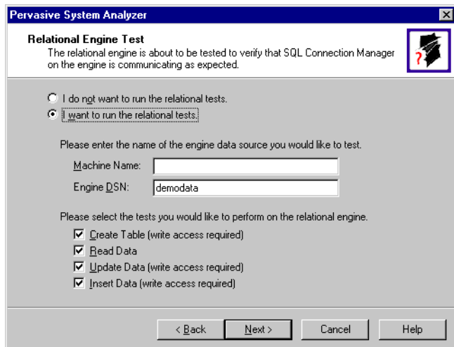
Figure 5-22 Relational Engine Test
