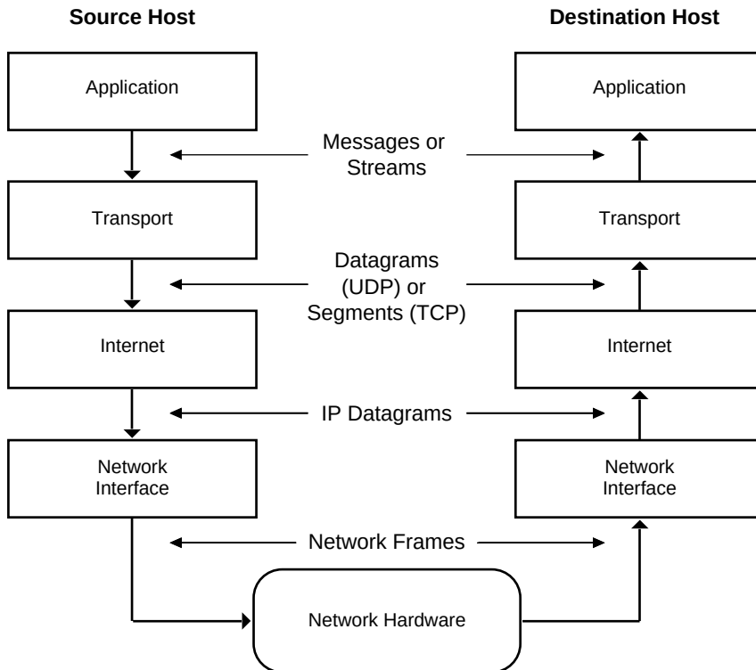
Figure 2 TCP/IP Model
