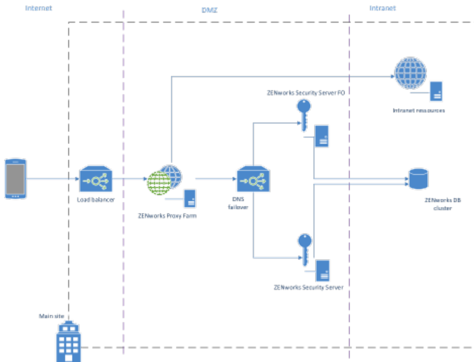
Figure 4. Load balancing
