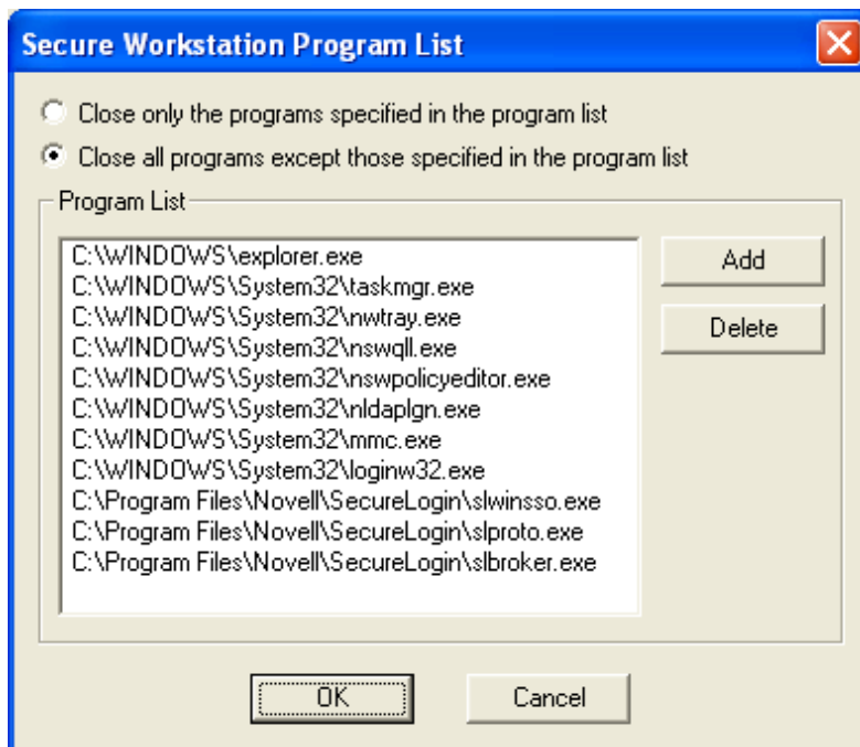
Figure 8-2 The program list dialog box
