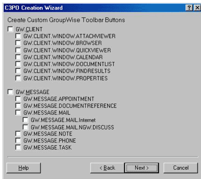
Figure 3-8 Toolbar Customization Screenshot
