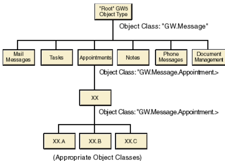
Figure 1-1 C3PO Object Class Hierarchy
