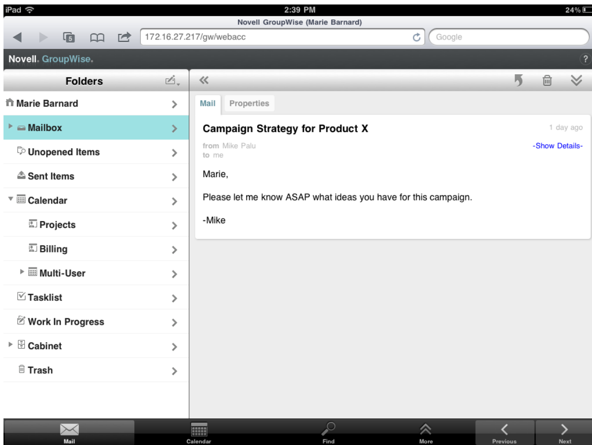
Figure 1-2 Folder List
