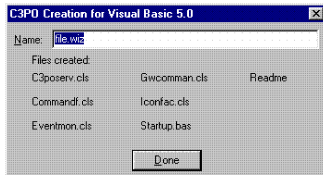
Figure 3-17 Completion Screenshot
