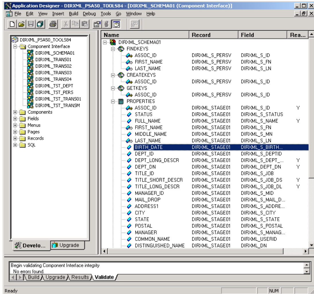
Figure 3-3 Schema Component
