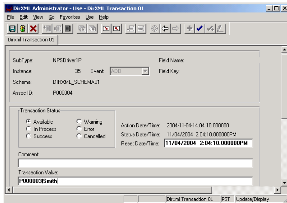
Figure 3-5 DirXML Transaction01
