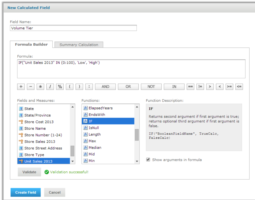
Figure 4-15 Formula Builder Tab in New Calculated Measure Dialog Box
