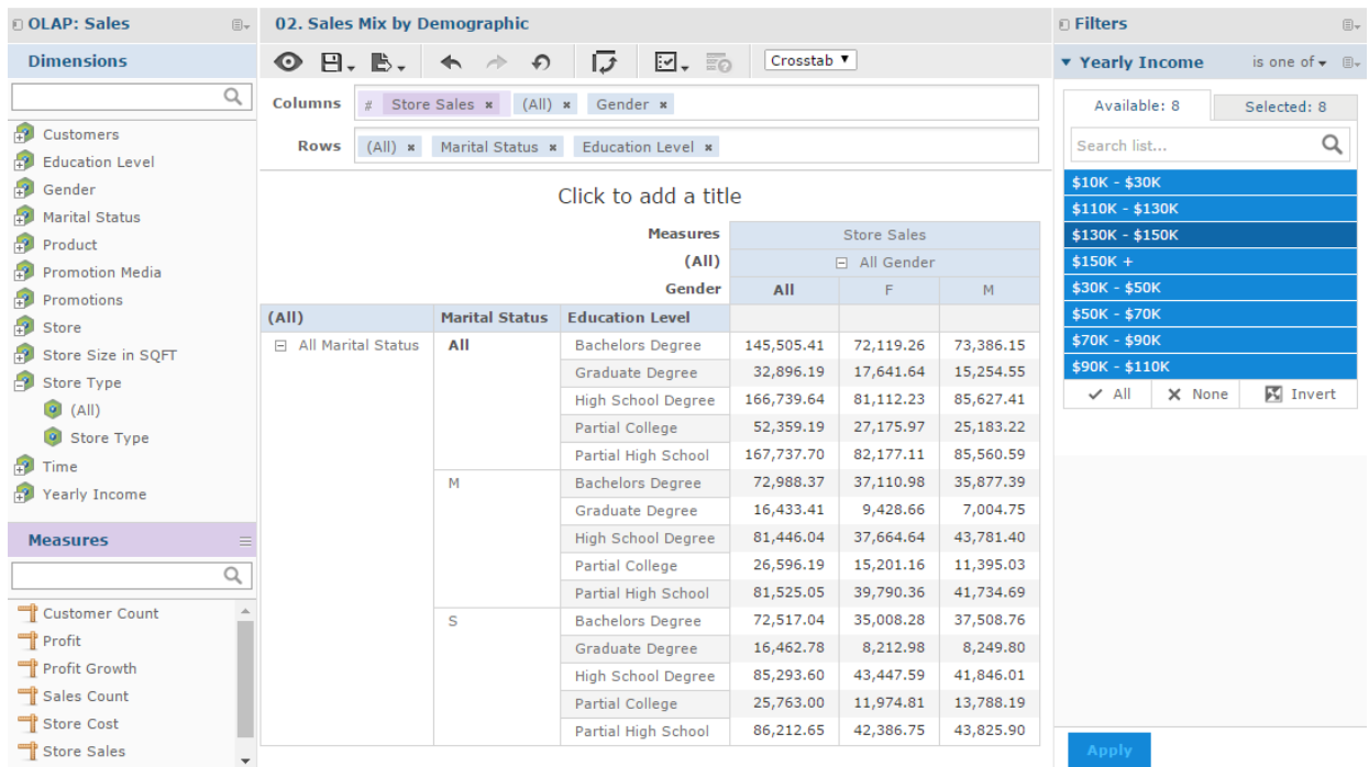
Figure 4-13 Ad Hoc Editor’s OLAP Connection-based Crosstab View
