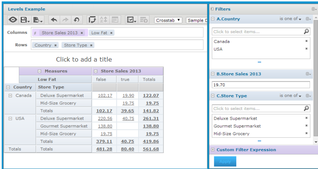
Figure 4-17 Base Example for Levels
