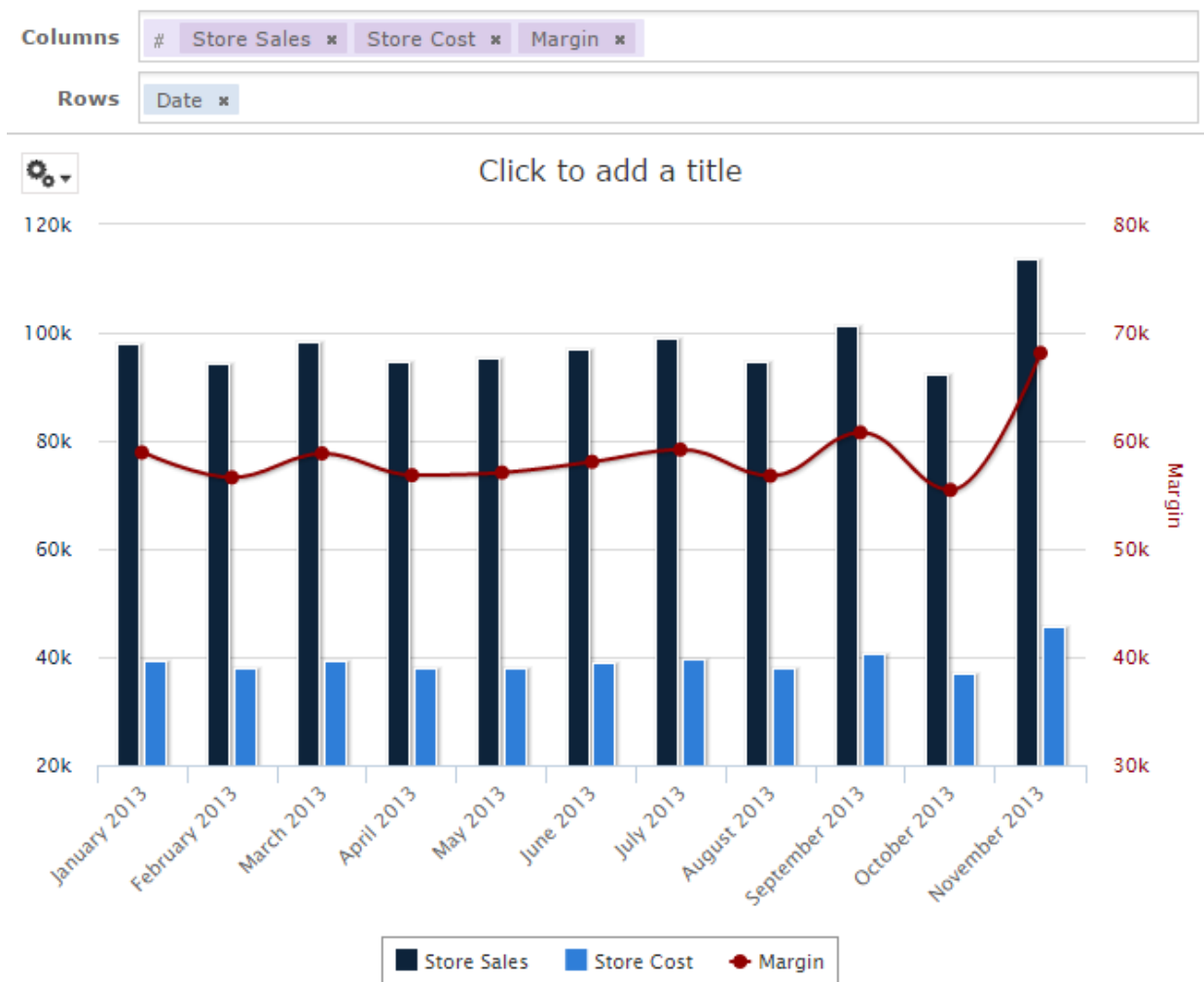
Figure 4-4 Ad Hoc Editor's Chart View
