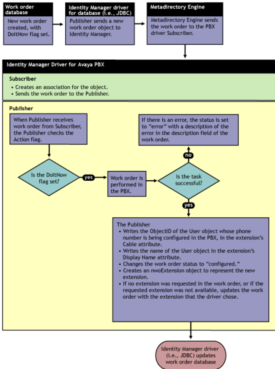
Figure 6-2 Flowchart of Work Order Database Configuration with the DoItNow flag Set to True
