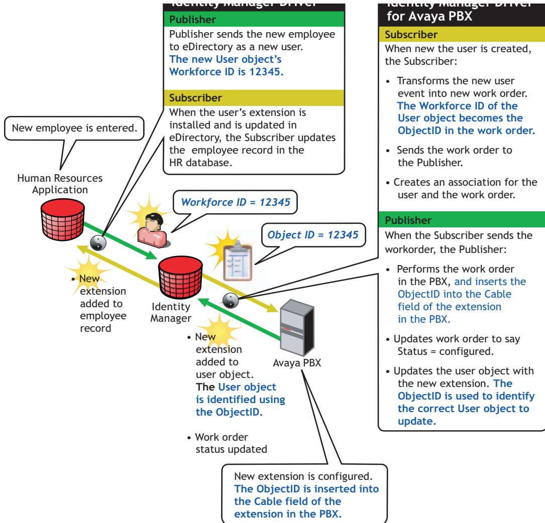
Figure 5-3 How the Object ID Is Used in the Process
