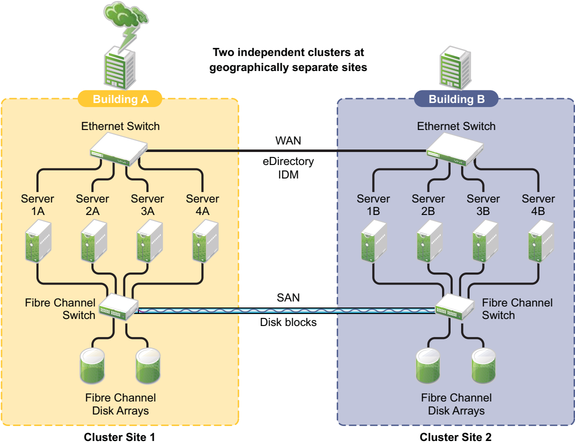
Figure 1-3 Two-Site Business Continuity Cluster
