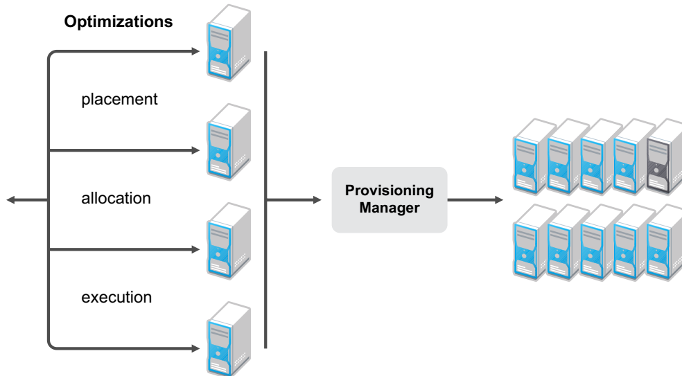
Figure 2-10 Workload Management
