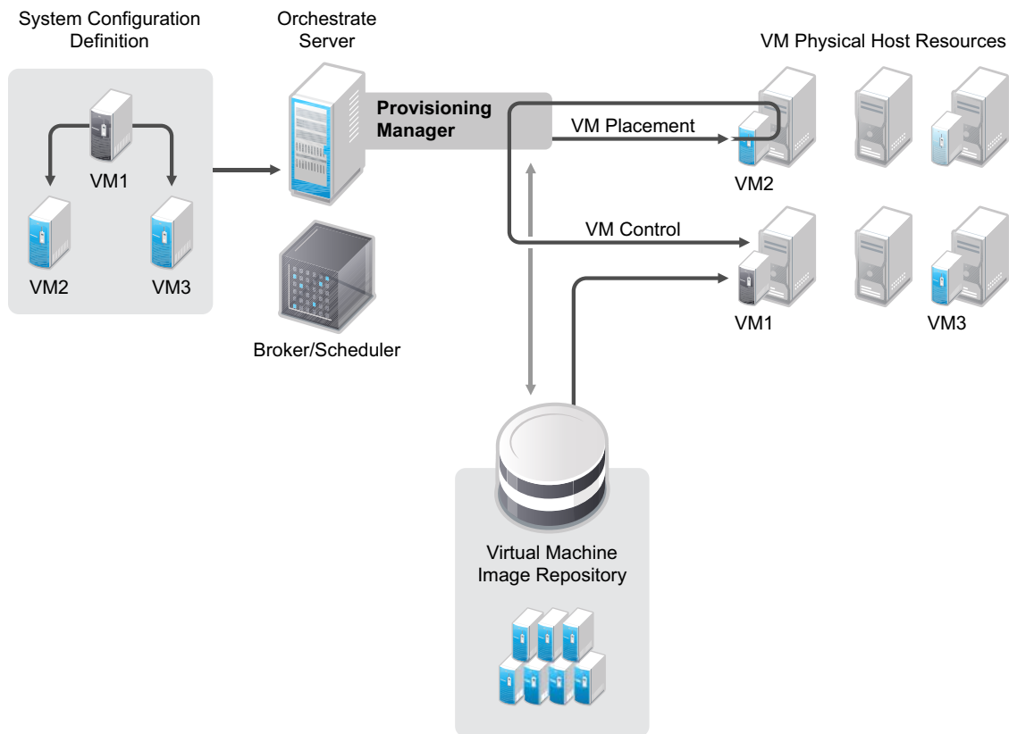
Figure 6-1 VM Management
