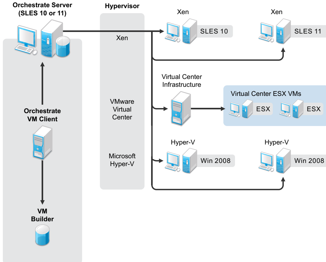
Figure 6-2 VM Management Provisioning Communications
