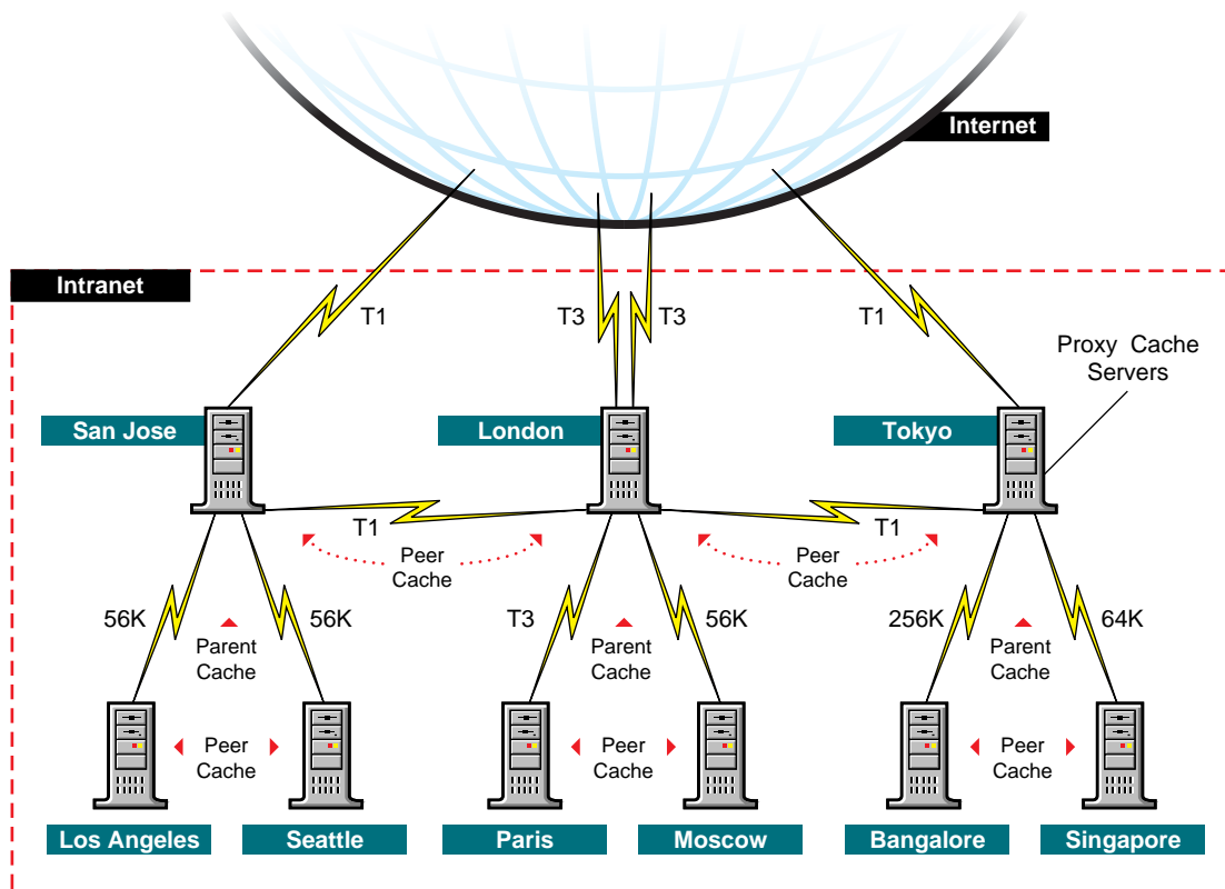
Figure 15 Intranet Network Accelerator Configuration Example
