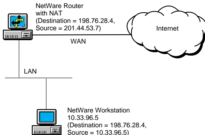
Figure 7 Dynamic Mode Implementation of NAT
