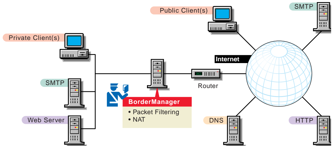
Figure 29 Using Novell Novell BorderManager 3.8 as an Address Translator
