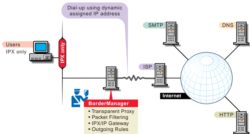
Figure 26 Connecting an IPX-Only Site to the Internet
