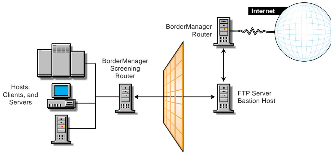
Figure 3 Screened Host Firewall
