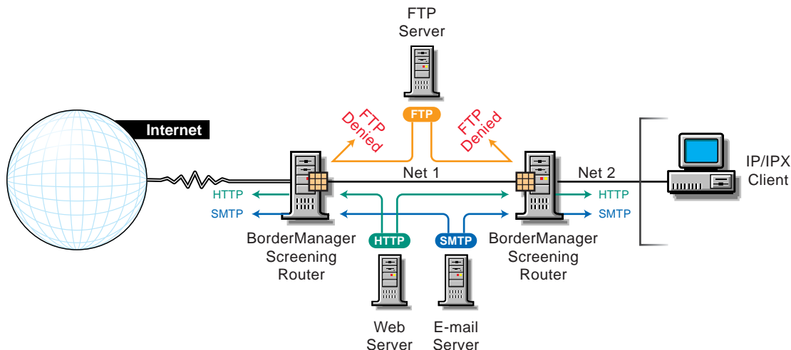
Figure 4 Screened Subnet Firewall
