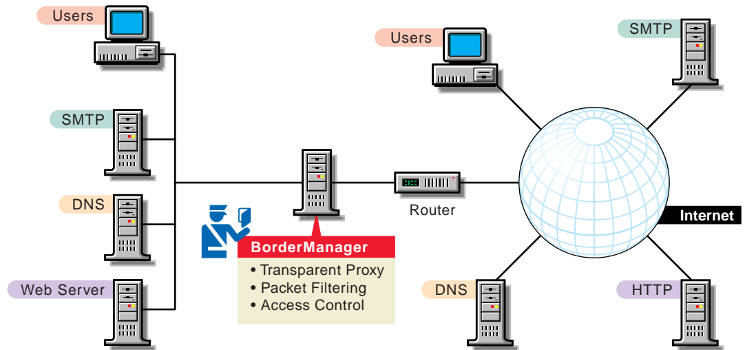
Figure 24 Inbound and Outbound Firewall
