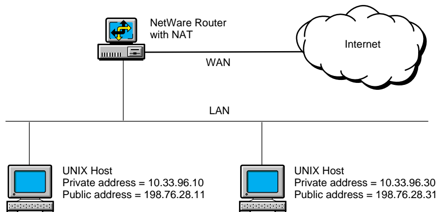
Figure 8 Static Mode Implementation of NAT
