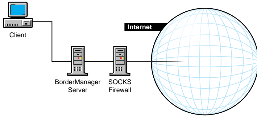
Figure 23 Novell BorderManager 3.8 Server behind a SOCKS Firewall
