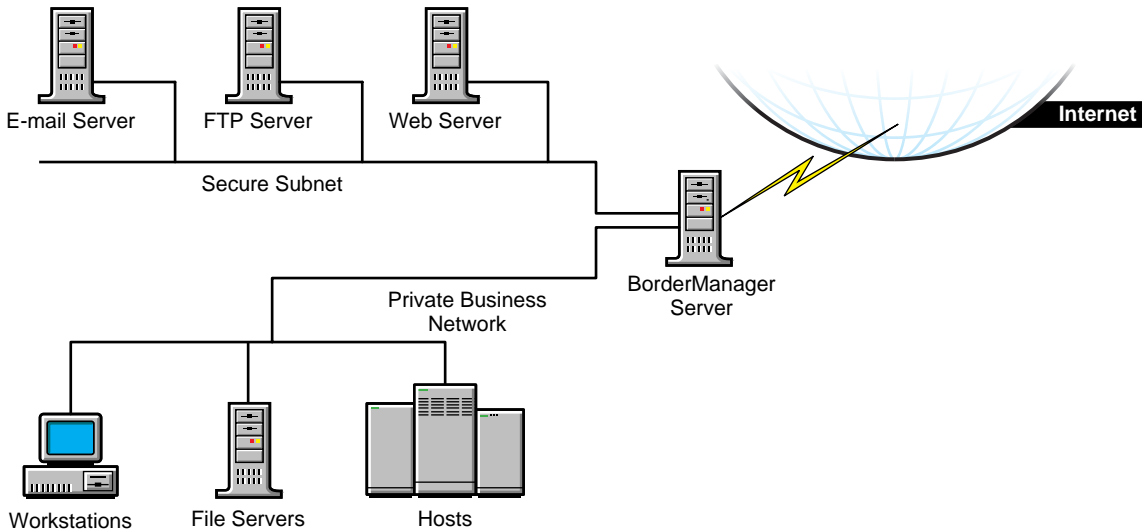
Figure 5 Tri-Homed Host
