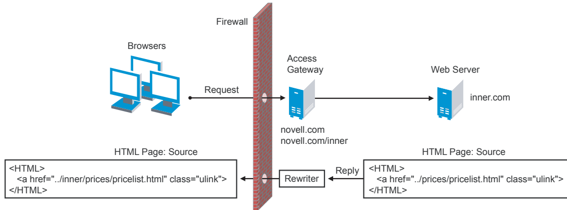
Figure 13-6 Rewriting with a Multi-homing Path
