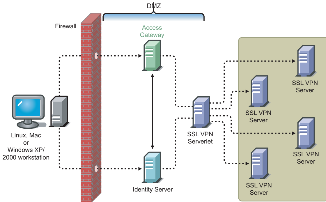
Figure 21-1 Load Balancing SSL VPN servers
