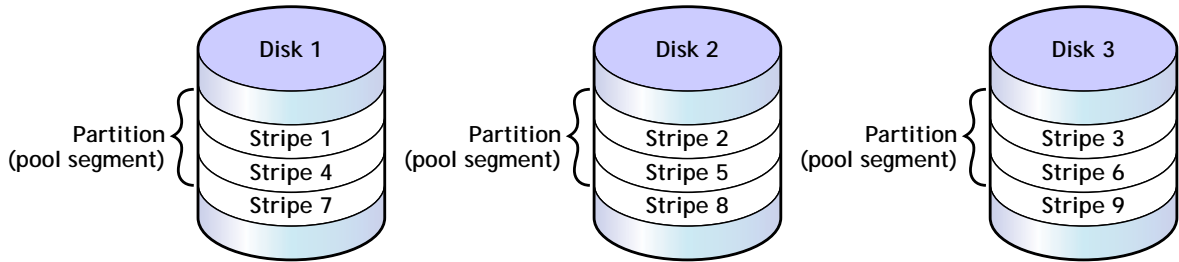
Figure 13-1 Striping Data on a Software RAID 0 Device
