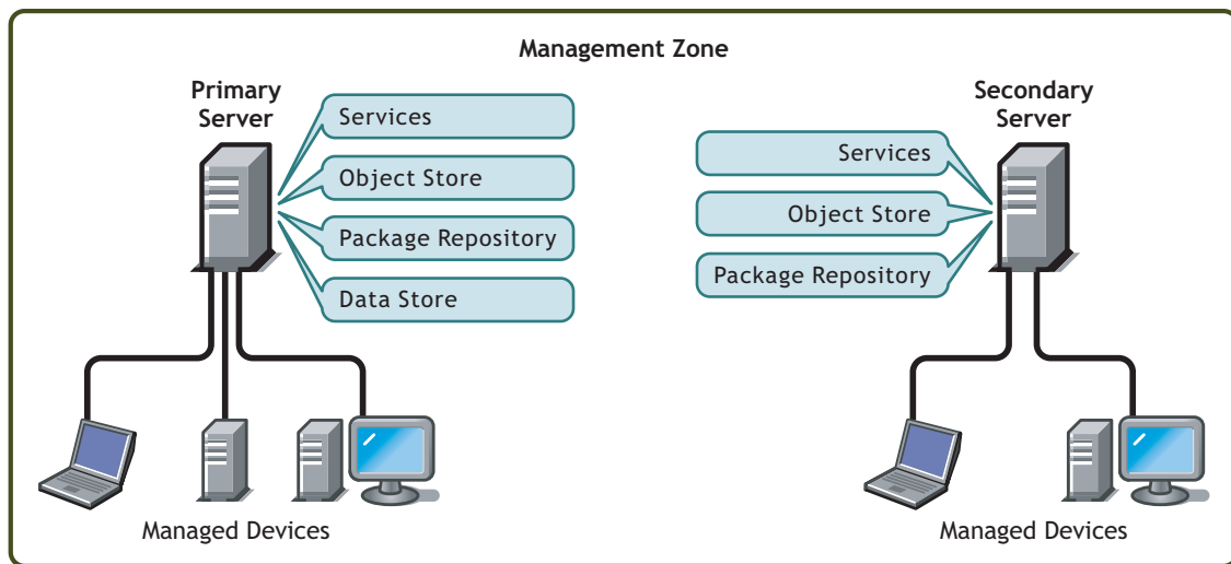
Figure 1-1 ZENworks Management Zone with a Primary Server, a Secondary Server, and Several Managed Devices
